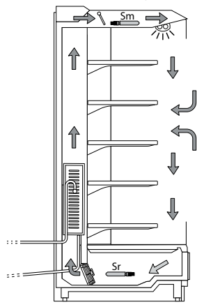
DAY: Sm = -21...-23 °C - Set point = -22 °C
