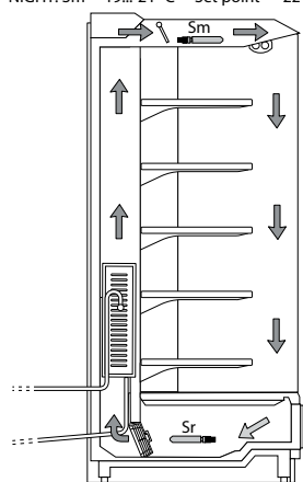
NIGHT: Sm = -19...-21 °C - Set point = -22 °C
